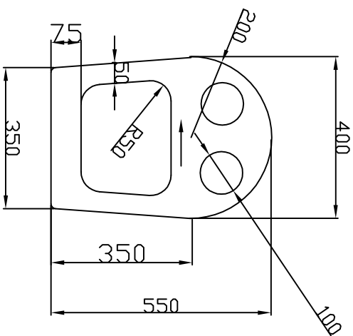
BULKHEAD 1 6MM BIRCH PLY
