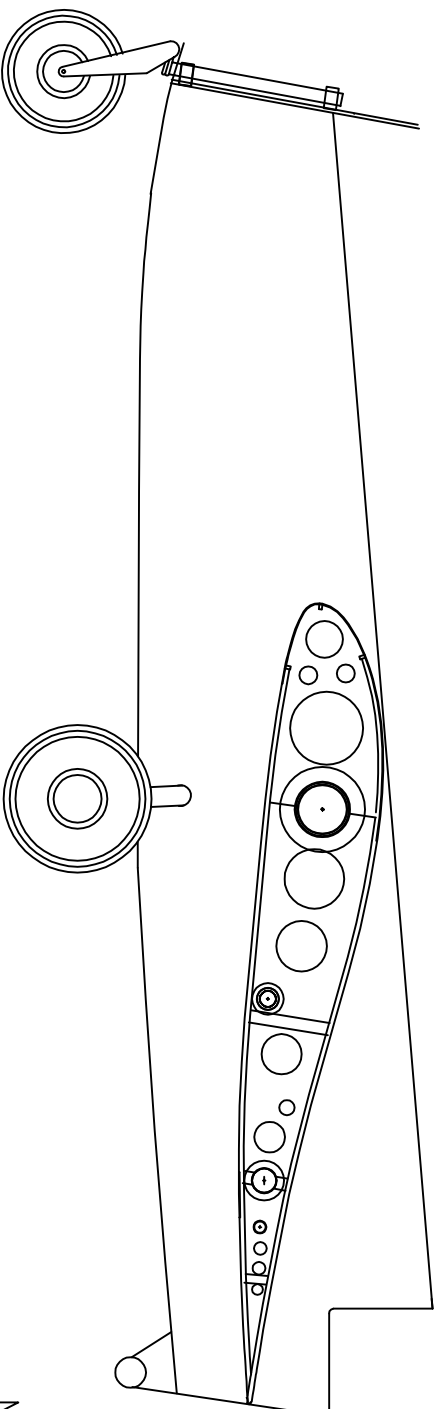
MW9B-22 WING CENTER SECTION
